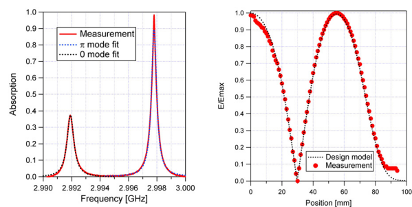
Figure 5: Frequency scan of the 1.6-cell RF-photogun showing two resonant frequencies, measured at 20 °C in air (left); Relative electrical field profile (right).
