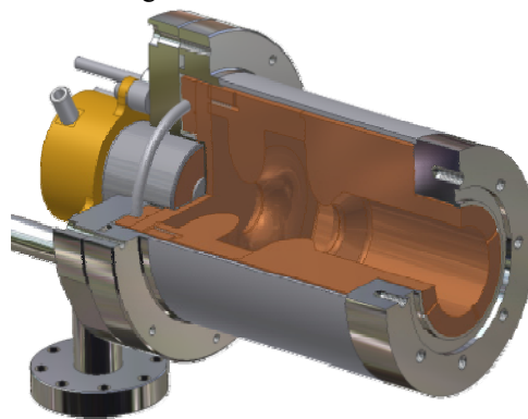
Figure 1: Schematic design of the 1.5-cell 2 nd generation Dutch RF-photogun.
