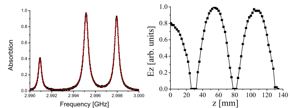
Figure 3: Frequency scan of the 2.6-cell RF-photogun (left) and field-profile of the \pi -mode (right).
