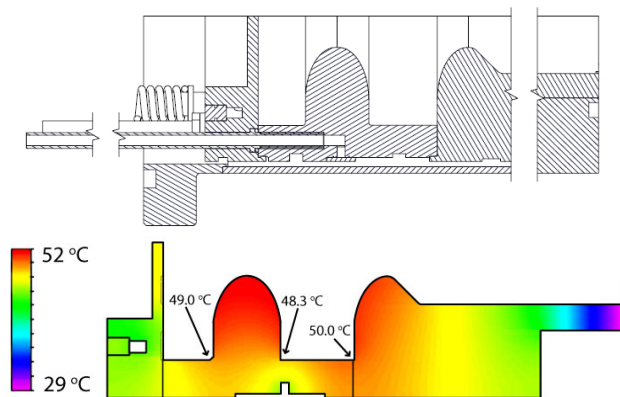
Figure 4: Detail of cross section of 1.6-cell. Cooling water channel with pipe connection and springs to clamp cavity (top). Temperature modeling of cavity with extra cooling channel (bottom).
