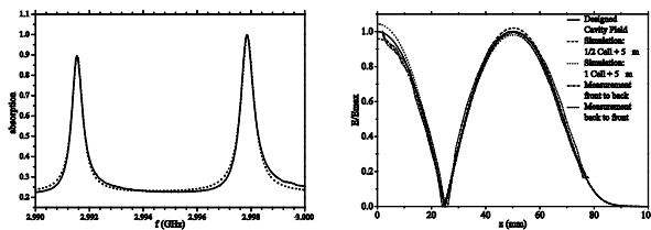
Figure 2: Frequency scan of the 1.5-cell RF-photogun showing two resonant frequencies, measured at 20 °C in air (top); Relative electrical field profile (bottom).
